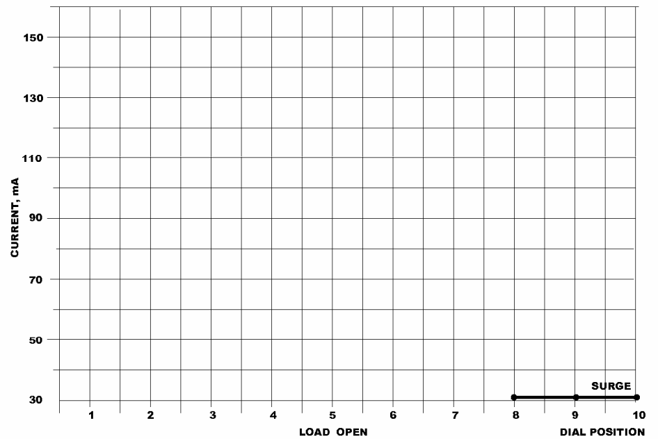
DISPERSIVE LEAKAGE vs DIAL POSITION
