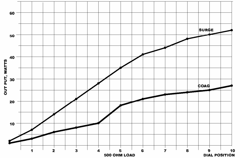
OUT PUT vs DIAL POSITION
