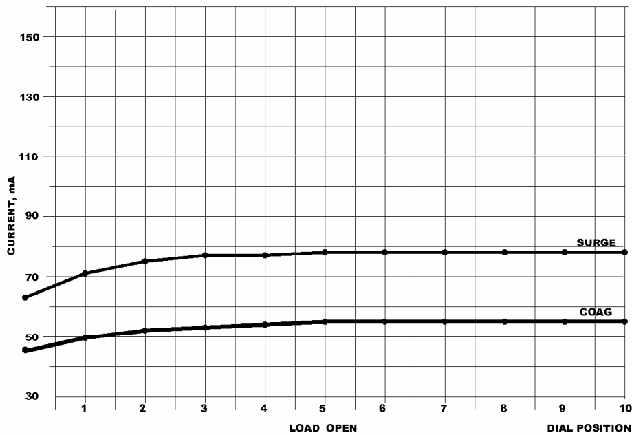
ACTIVE RF LEAKAGE vs DIAL POSITION
