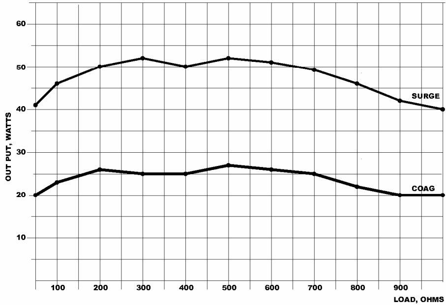
MAXIMUM OUTPUT vs LOAD
